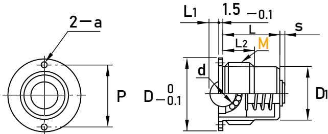
BCHPT (External thread type)
