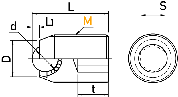
(BCSB stainless steel ball)
